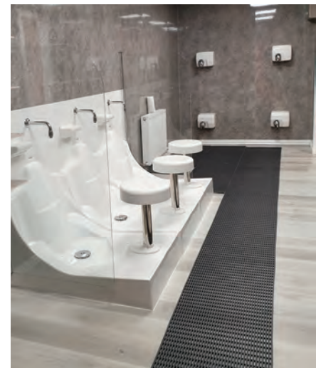
WUDUMATE MODULAR WITH NON-SLIP MATTING & FOOT DRYERS
